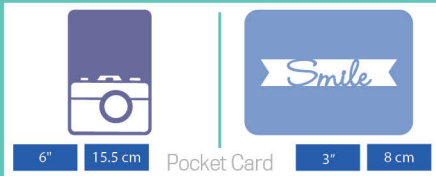
Sentiment
